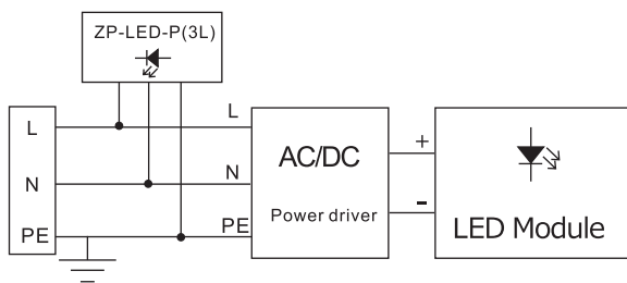
Single-phase connection
