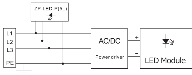
Three-phase connection
