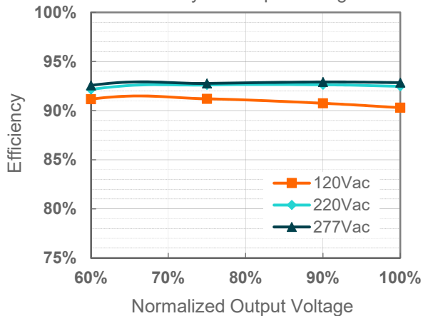
EUM-150S150Dx (Io=1050mA)
