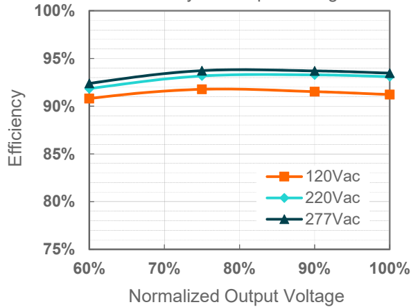
EUM-150S105Dx (Io=700mA)
