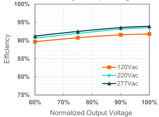
EUM-150S105Dx (Io=1050mA)
