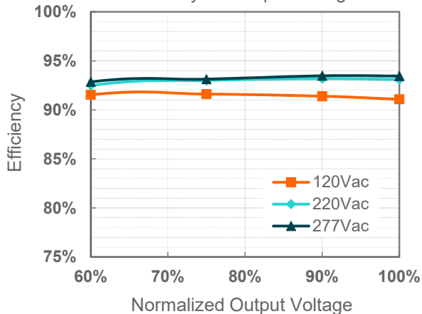
EUM-150S150Dx (Io=1050mA)
