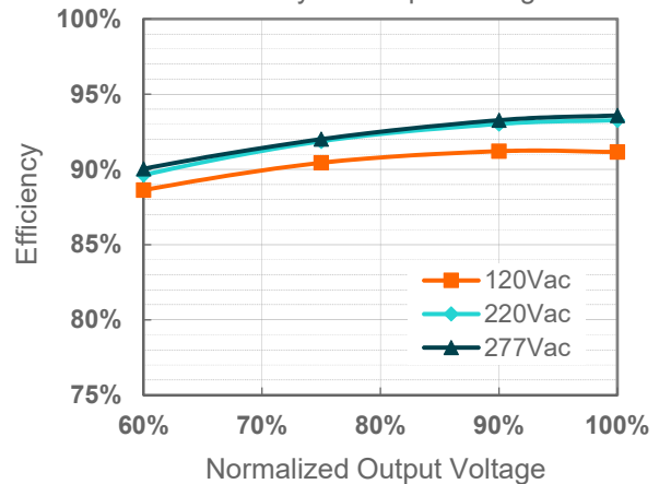
EUM-150S150Dx (Io=1500mA)
