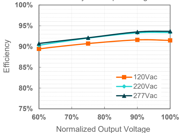
EUM-150S150Dx (Io=1500mA)
